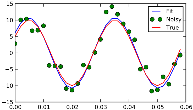
Least-squares fit to noisy data
