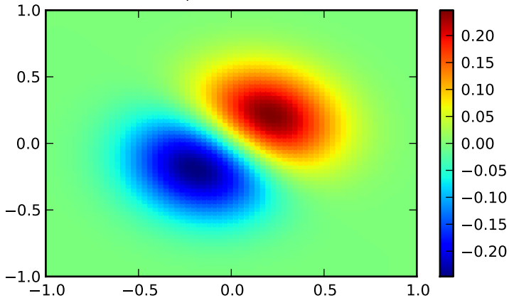
Interpolated function.
