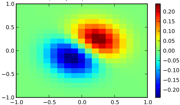
Sparsely sampled function.
