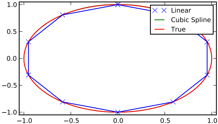
Spline of parametrically-defined curve
