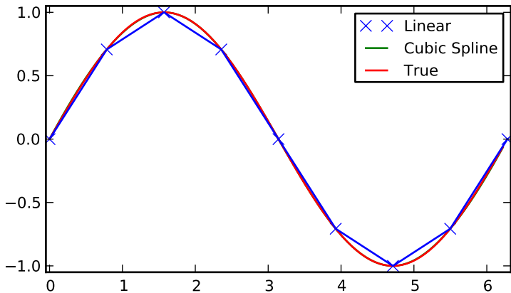
Cubic-spline interpolation
