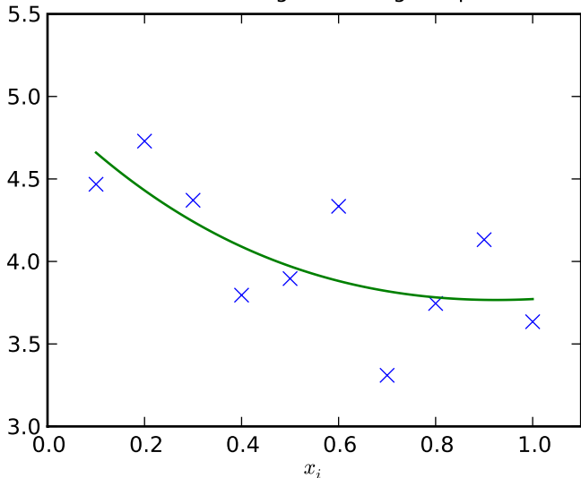
Data fitting with linalg.lstsq
