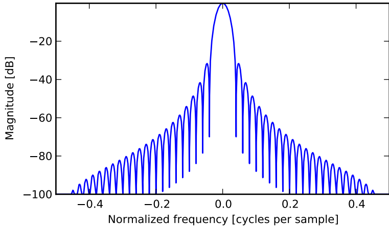
Frequency response of the Hann window
