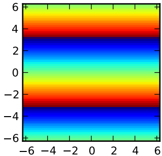
Phase (angle) of \exp(x)
