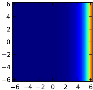
Magnitude of \exp(x)
