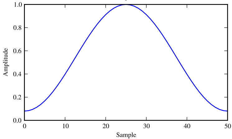
Hamming window
