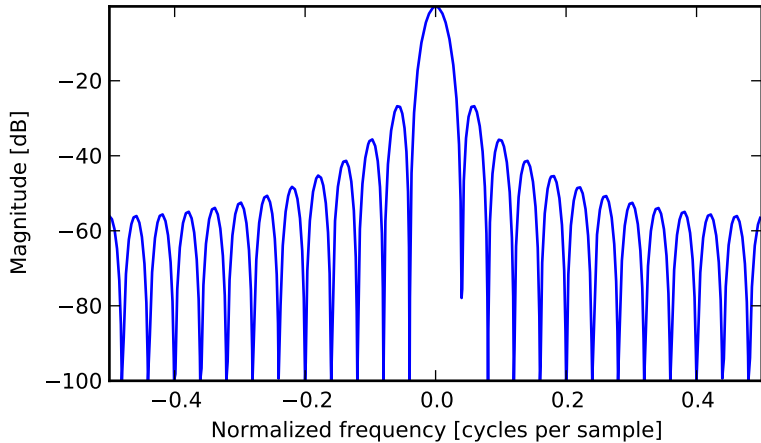
Frequency response of Blackman window
