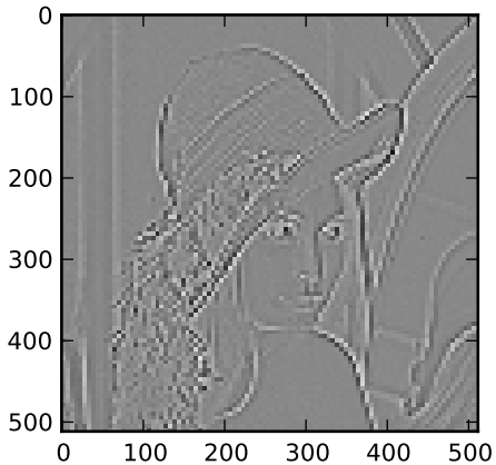
Output of spline edge filter
