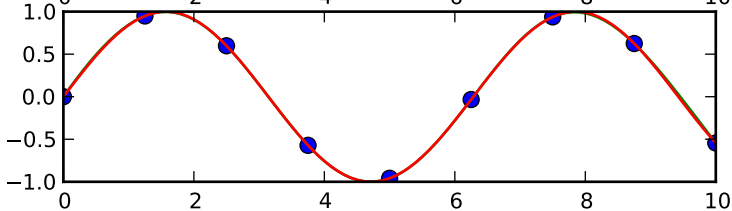
Interpolation using RBF - multiquadrics
