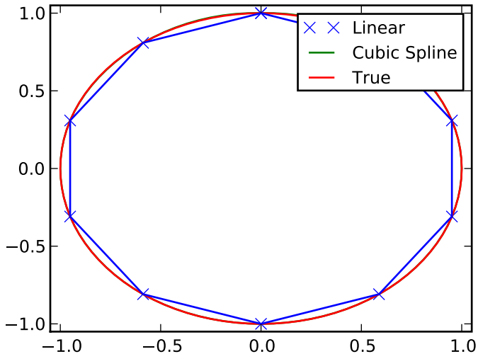
Spline of parametrically-defined curve
