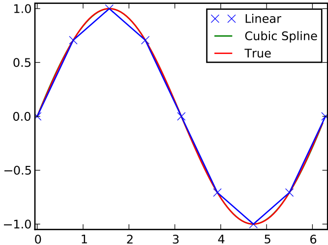
Cubic-spline interpolation
