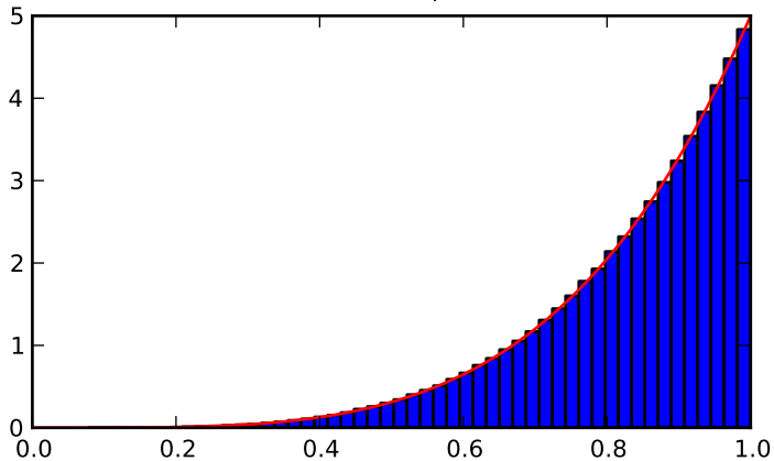
inverse of stats.pareto(5)
